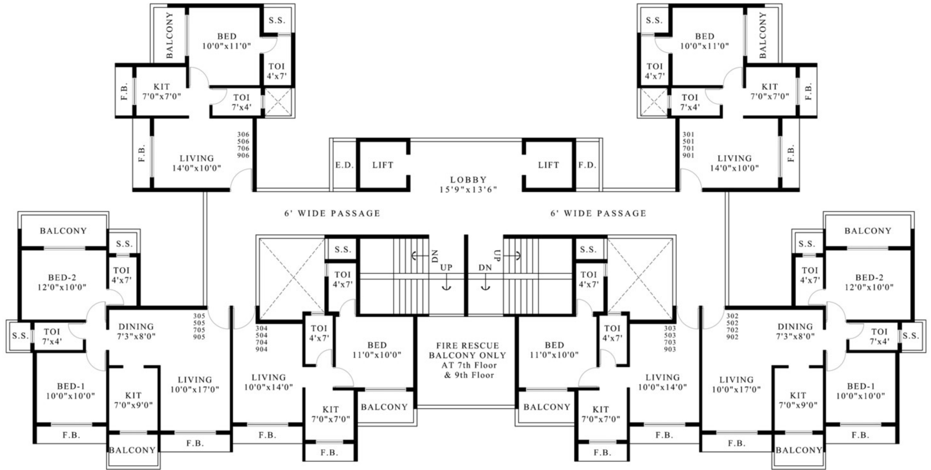
ODD-Floor Plans
