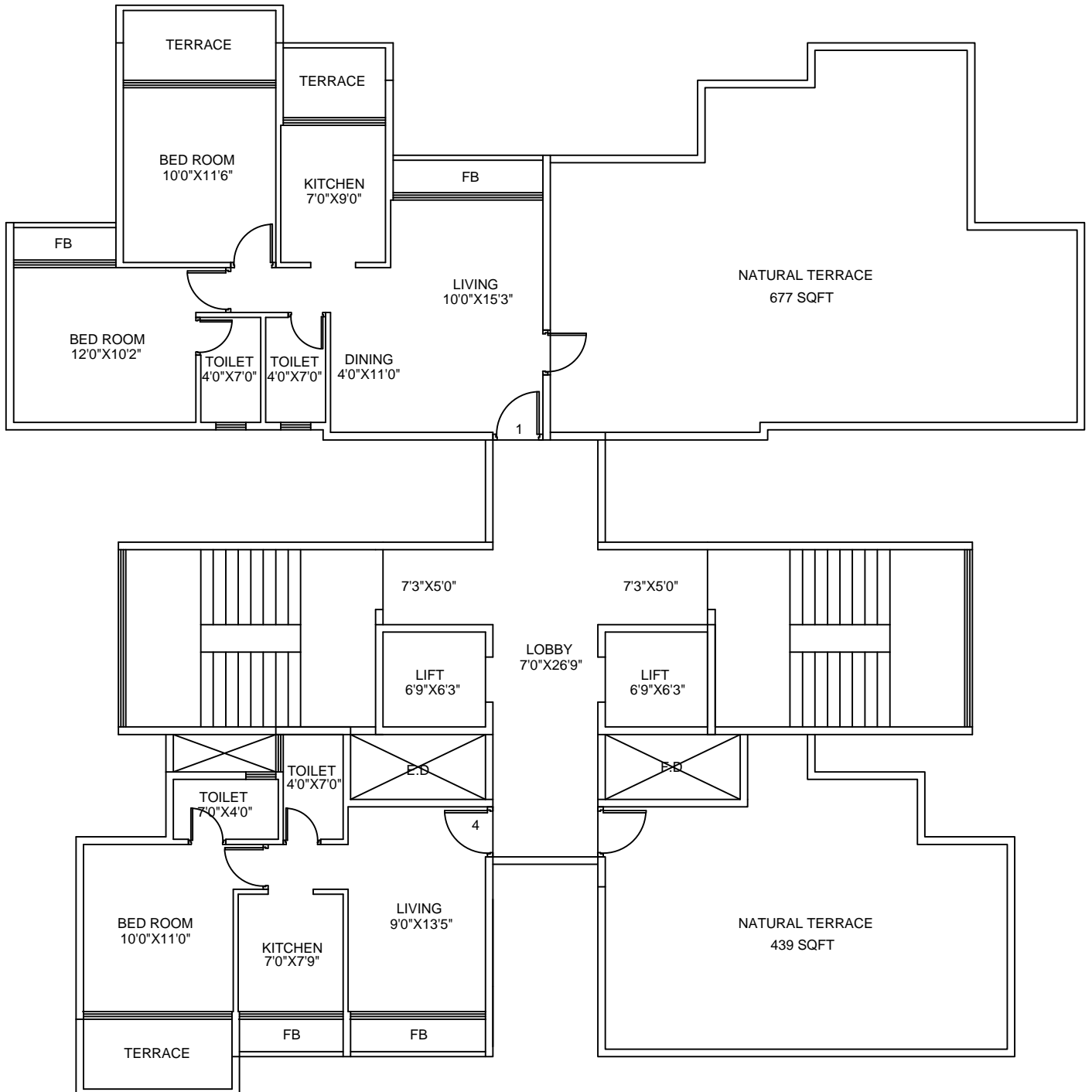
14TH FLOOR PLAN
