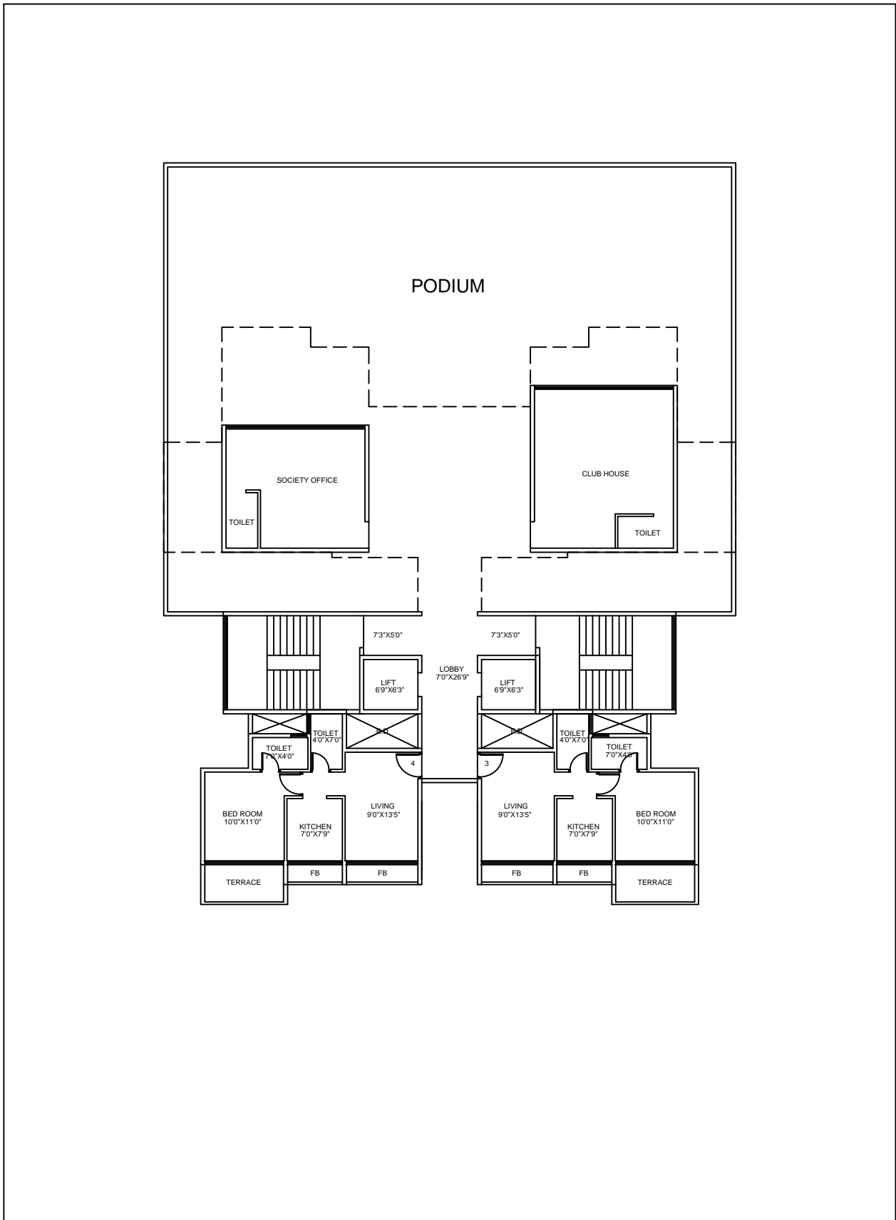
2ND FLOOR PLAN
