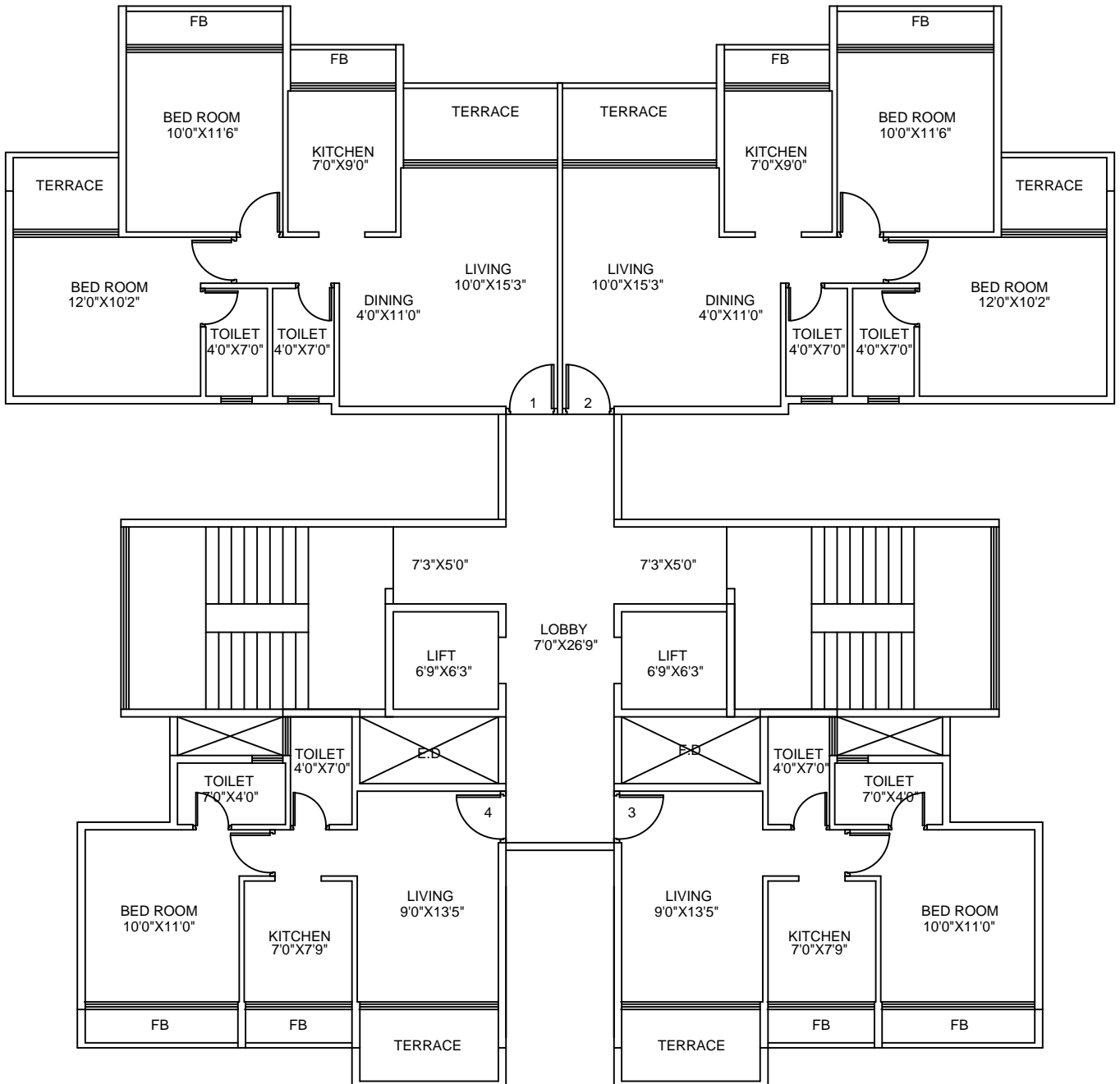
TYPICAL FLOOR PLAN ODD FLOORS 3,5,7,9,11,13
